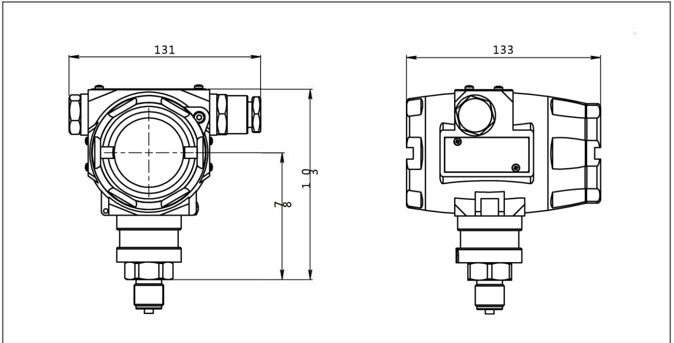
Drawing and dimension of GI 305X-TST-S with display(C) (unit: mm)
