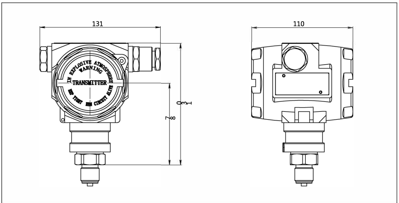
Drawing and dimension of GI 305X-TST-S without display(A) (unit: mm)
